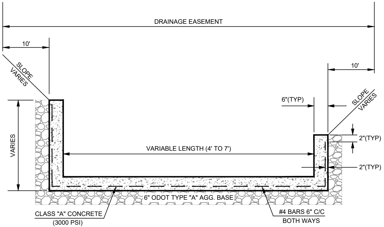
TYPICAL CHANNEL DETAIL
