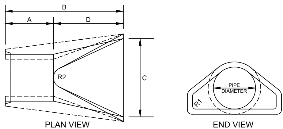
ROUND CONCRETE END SECTION
