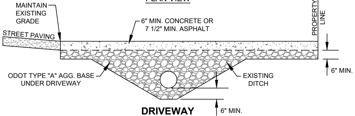
DRIVEWAY PLAN VIEW
